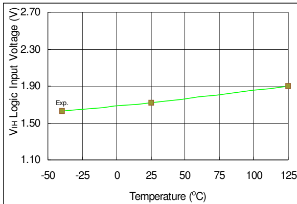
Figure 31. V IH Logic Input Voltage vs. Temperature
